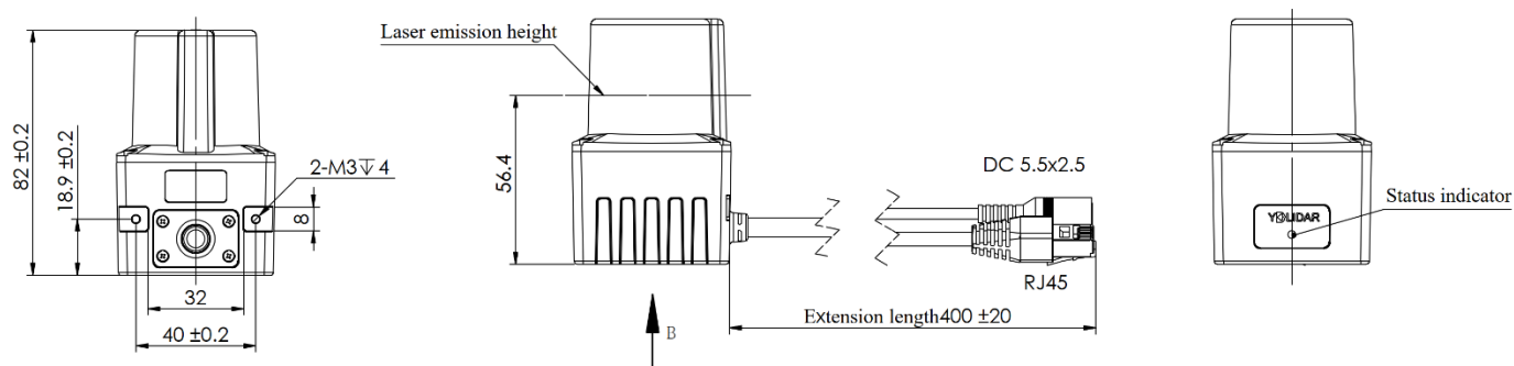
FIG 2 YDLIDAR TIA MECHANICAL DIMENSION (UNIT:MM)
