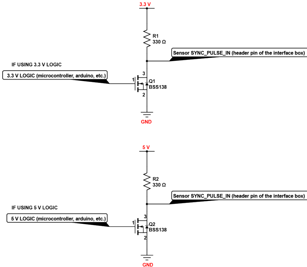
Figure5.2: Example Circuits for 3.3 V and 5 V logic
