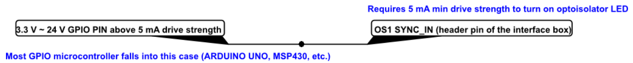
Figure5.1: Example Circuits for 3.3 V and 5 V logic
