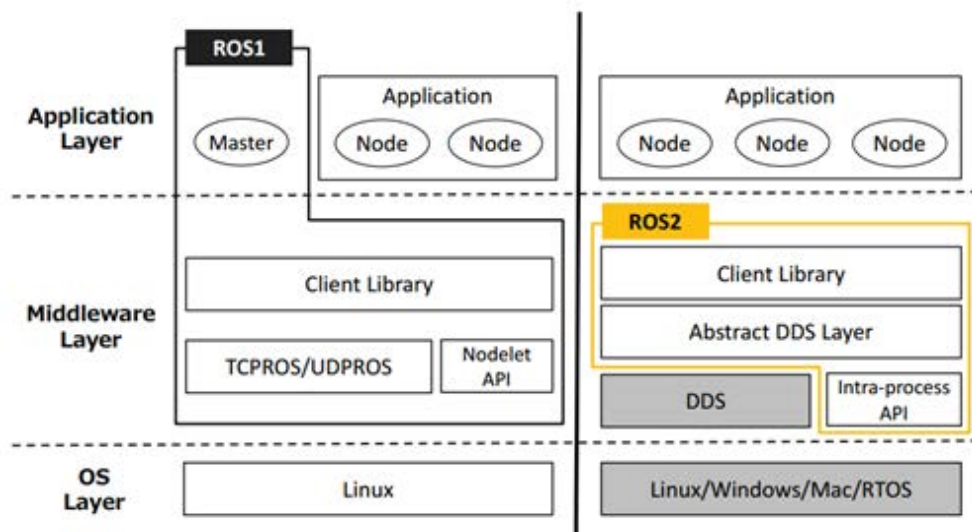
Figure 1: ROS1/ROS2 architecture.
